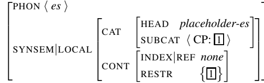
Figure 6: Lexical entry for expletive placeholder es (preliminary)
